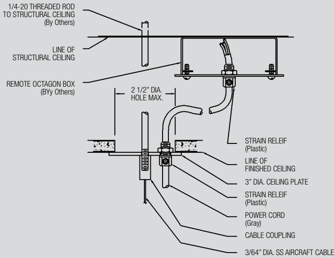
OPTIONAL SUPPORT CABLE/FEED OPTION: WS-2
