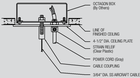
STANDARD SUPPORT CABLE/FEED OPTION: WS-1
